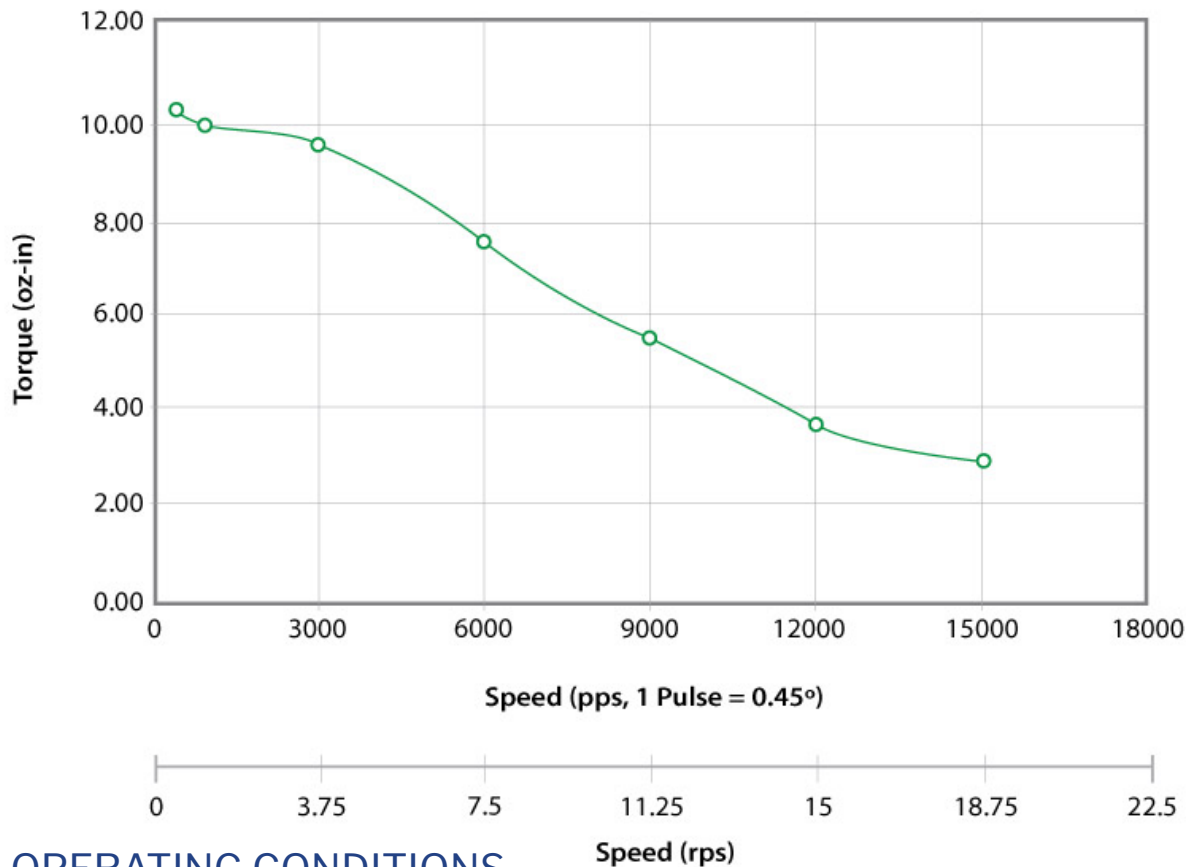
Z417-11-18 (0.9° Step Motor) 24VDC, 0.6 Amp/Phase, Bipolar, 1/2 Stepping
